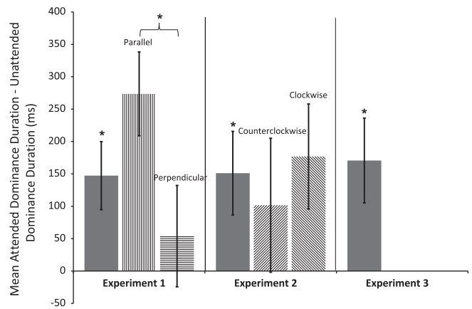
Fig. 3. Differences in dominance period length. In Experiment 1, the overall effect of attention is a significant increase in dominance duration for the attended stimulus (solid bar). This effect is driven by the trials where the two surfaces contain stripes parallel to the overlapping frames (vertical pattern), and greatly reduced in trials containing perpendicular stripes (horizontal pattern). Experiments 2 replicates this effect of attention with afterimages oriented obliquely to the frames. While the effect across all trials (solid bar) is similar to Experiment 1, there is no significant effect of stripe orientation in Experiment 2 (diagonally-striped bars). Experiment 3 replicates the difference between attended and unattended afterimages with completely overlapping afterimage patterns and attention cued to a feature of the afterimages themselves. All error bars represent SEM.
